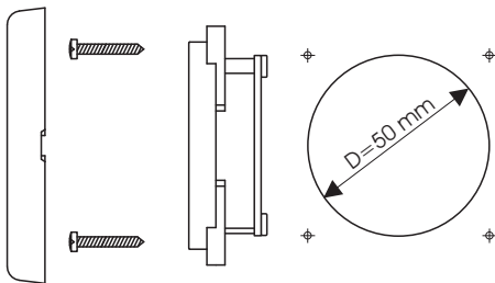
Fissaggio ad incasso Built-in fixing Wandeinbau Fixation encastrée
