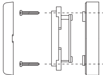
Fissaggio a parete Wall-fixing Wandbefestigung Fixation murale
